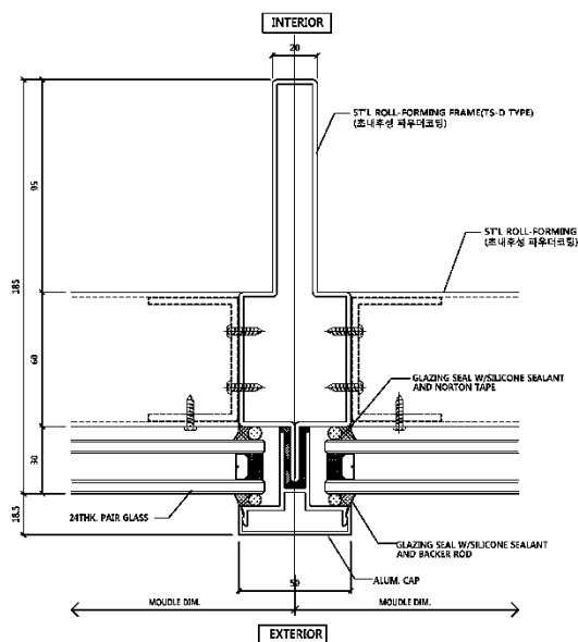
1 D1 HORIZONTAL SECTION VIEW OF STRUC. MULLION
