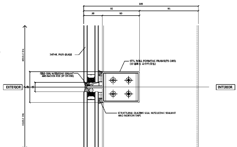
2 D1 VERTICAL SECTION VIEW OF VISION TRANSOM
